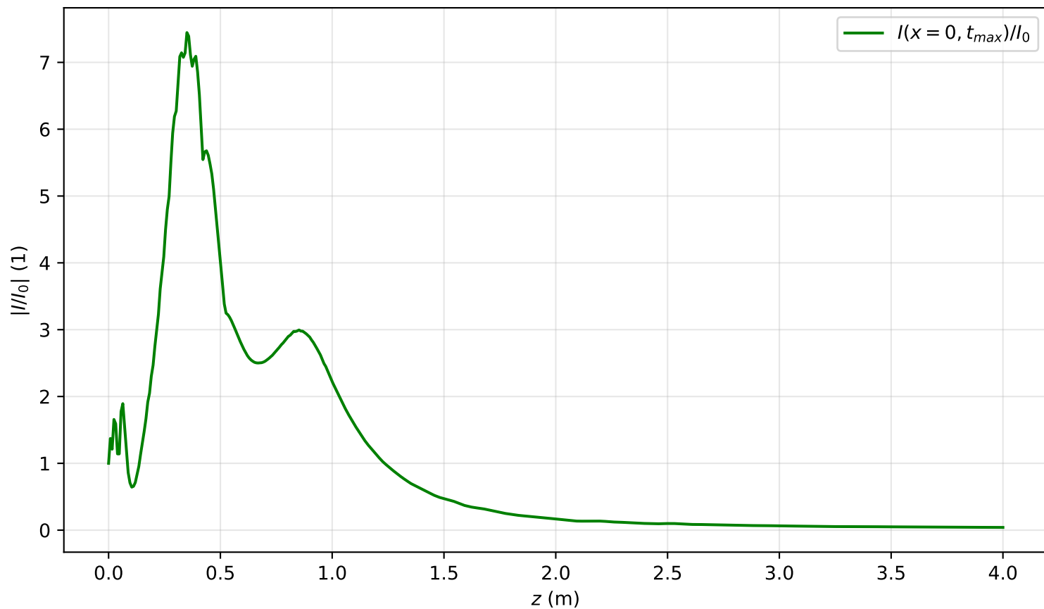
I(x=0, t_{max}, z)/I_0 , Pin=4.1Pcr
